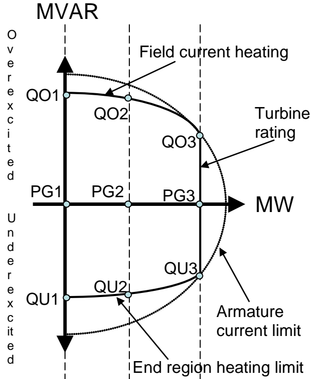
Figure 1 - Typical Generator Capability Curve
