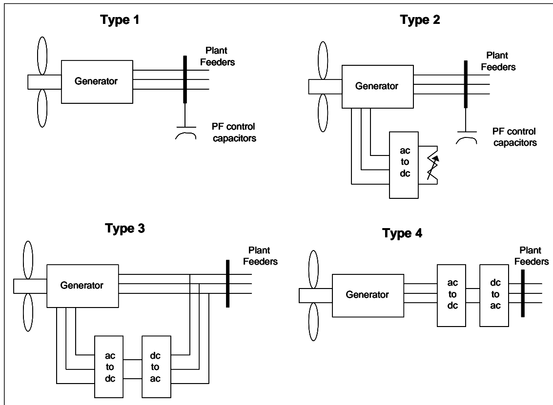
Figure C-3 - Four Basic Wind Turbine Topologies
